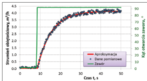
Rys. 4. Charakterystyka skokowa z badań dla procedury OE (przetwornik \tau = 7 s) Fig. 4. Jump characteristic from the tests for the OE procedure (transducer \tau = 7 s)
